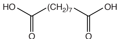
azelaic acid
